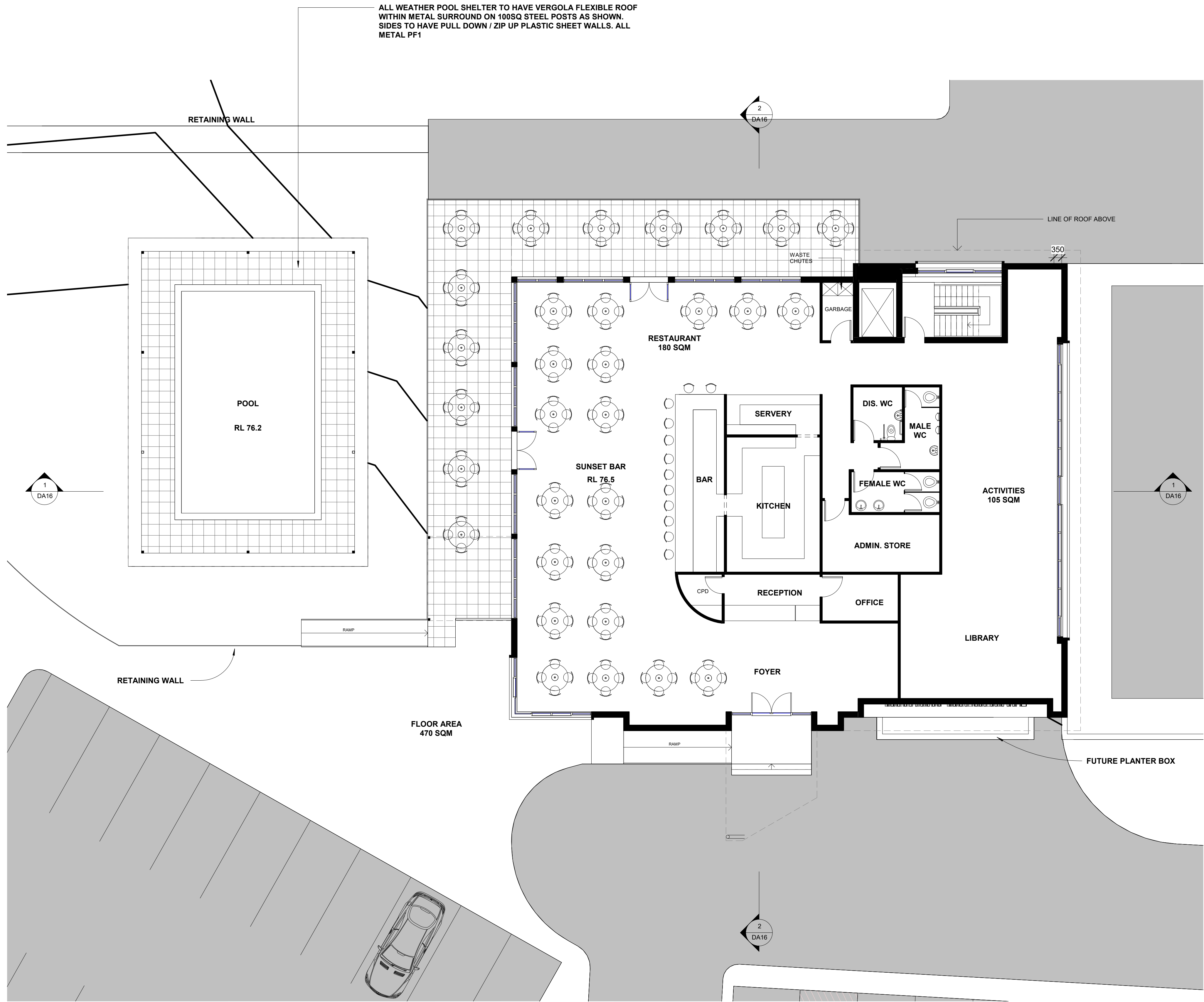
1 GROUND FLOOR PLAN 1 : 100
